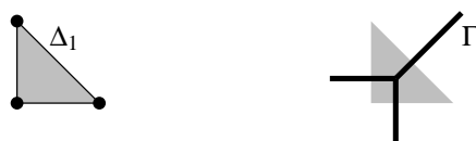
FIGURE 5. Tropical lines are “dual” to \Delta_1
